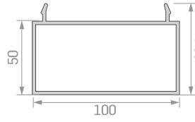
1790 Kapaklı Kolon Alt Profili COLUMN BELOW PROFILE WITH COVER Ağırlık / Weight: 1,976
