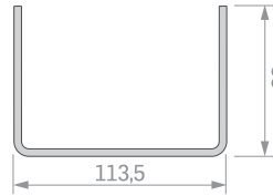
1745 Kare Kolon İçi U Profil SQUARE COLUMN INSIDE U PROFILE Ağırlık / Weight: 2,821
